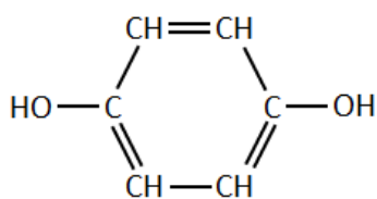
hydroquinone
